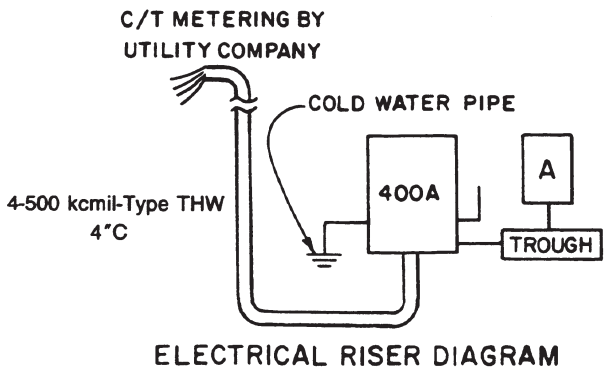
ELECTRICAL RISER DIAGRAM
