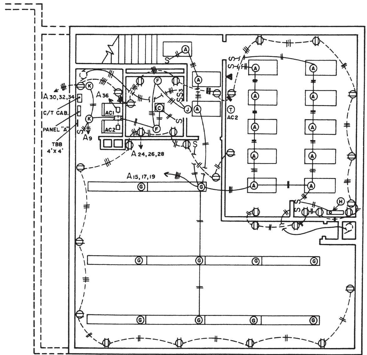
BASEMENT LIGHTING AND POWER PLAN SCALE 1/8" = 1'-0"
