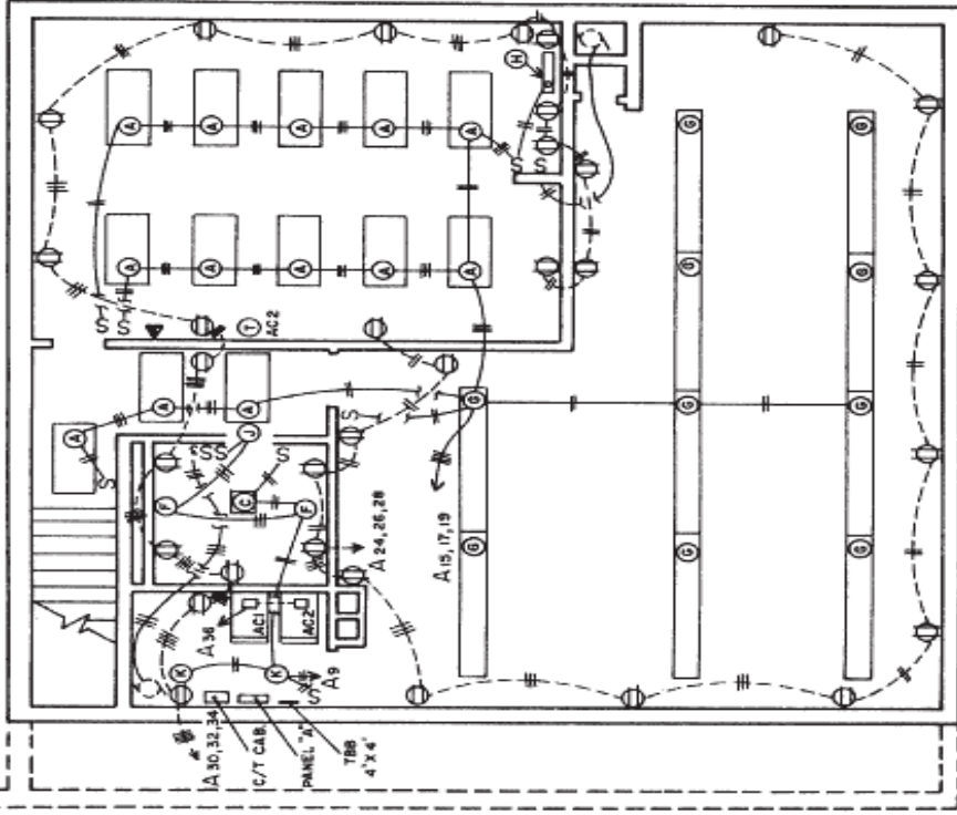
BASEMENT LIGHTING AND POWER PLAN SCALE 1/8"=1'-0"
