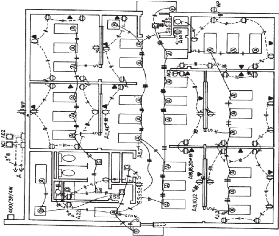
FIRST FLOOR LIGHTING & POWER PLAN SCALE 1/8"=1'-0"
